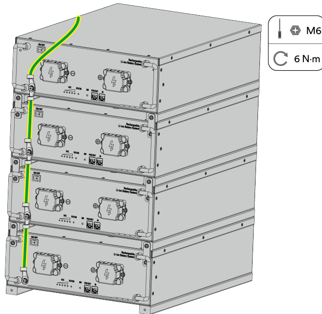
2-4 modules connection
