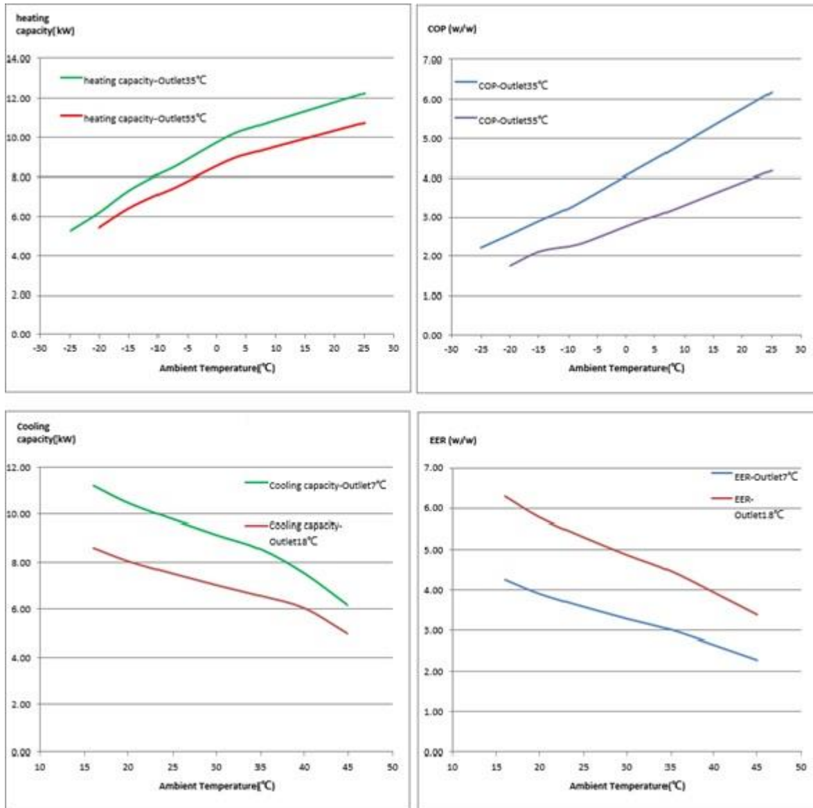
SOL-010HC3 Heating performance graph
