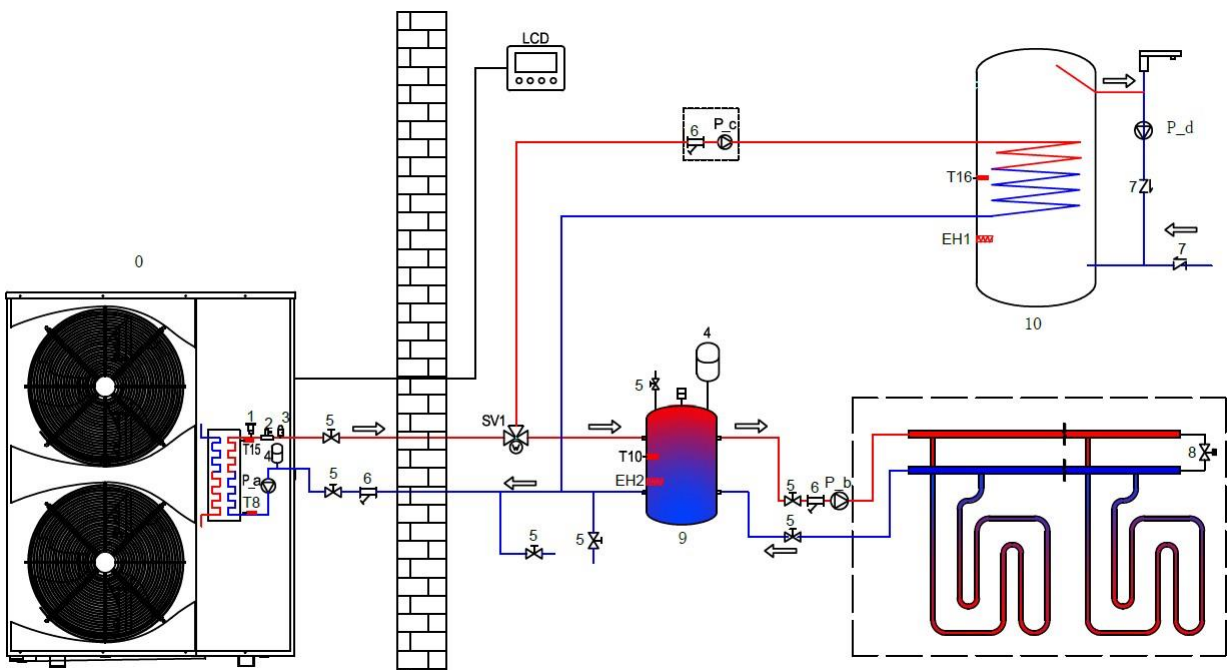
3.7.5 Installation diagram of hot water + floor heating mode waterway system
