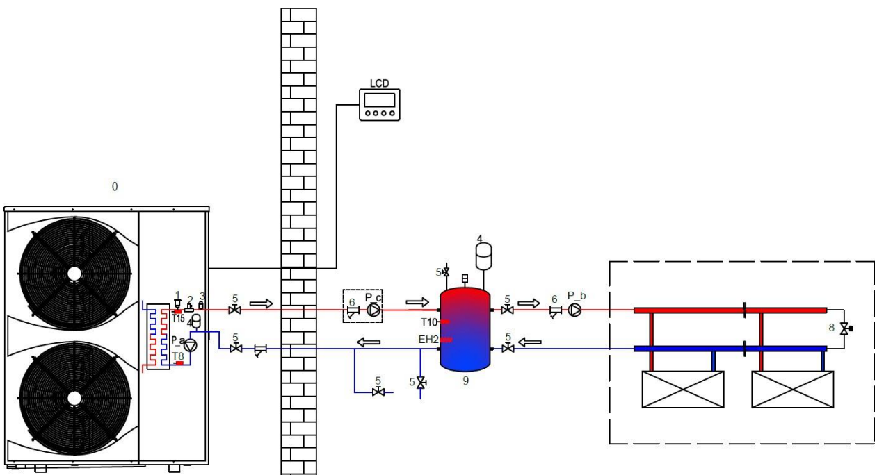
Installation diagram of the heating or cooling mode waterway system
