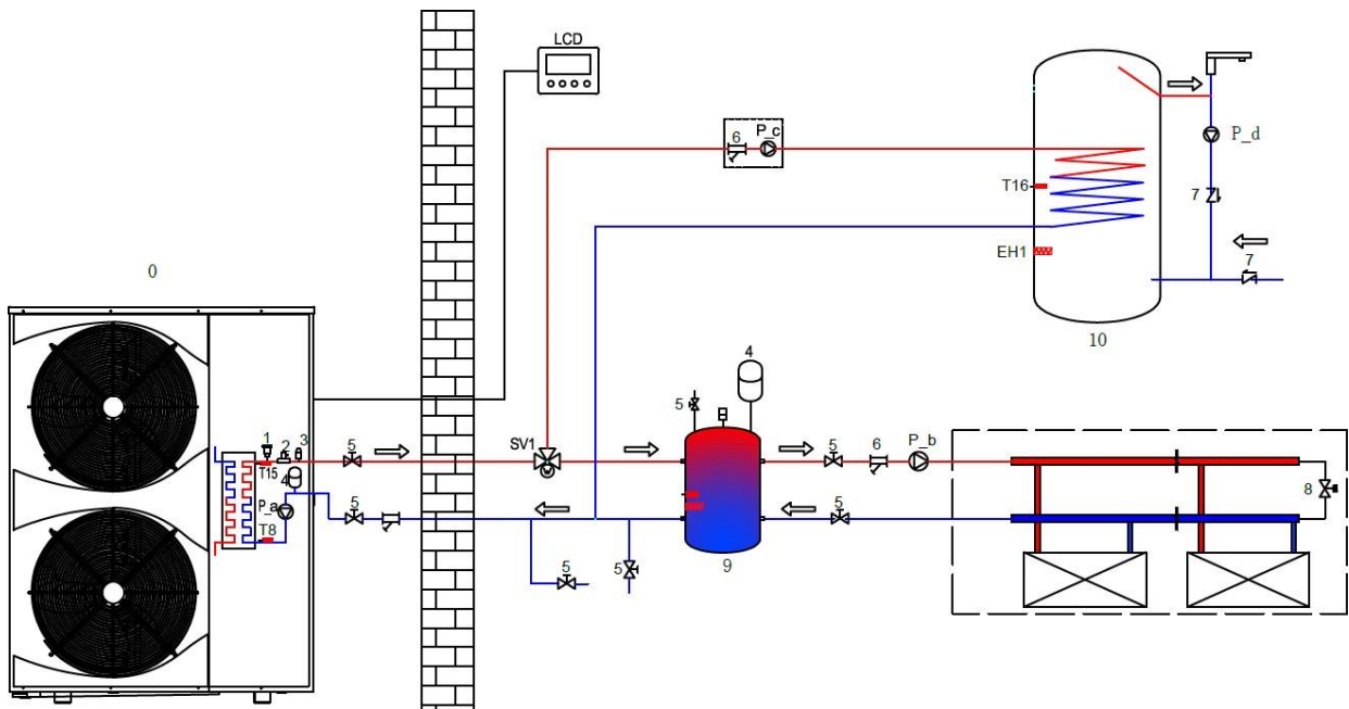
3.7.5 Installation diagram of hot water + floor heating mode waterway system
