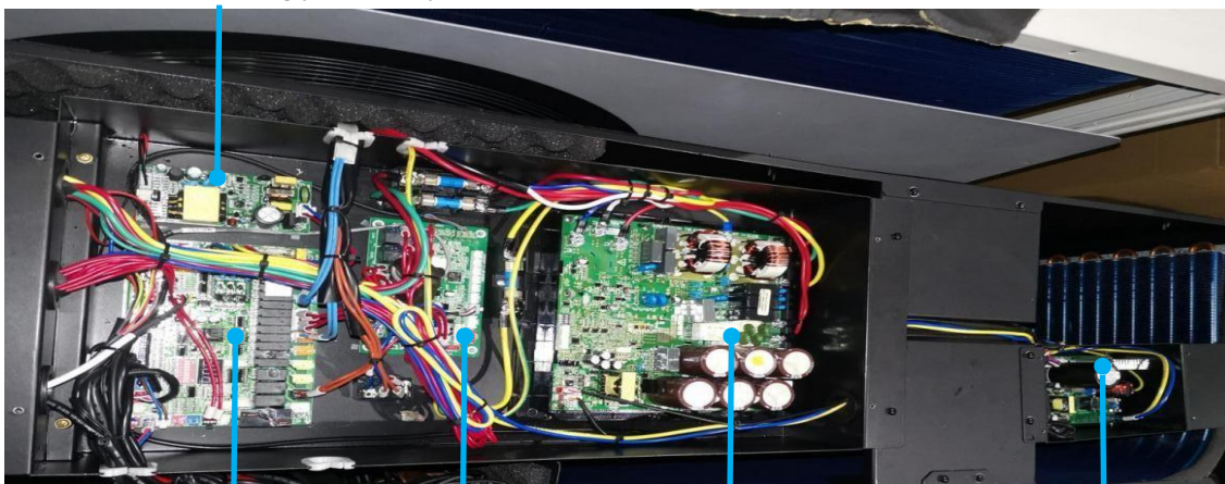
AP2 Switching power strip PCB
