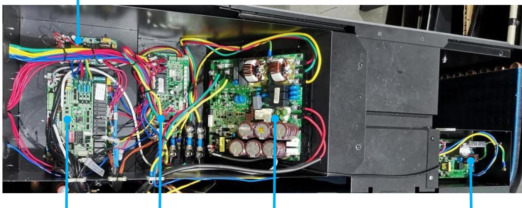
AP2 Switching power strip PCB
