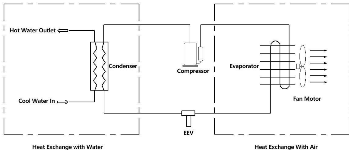
Working principle diagram
