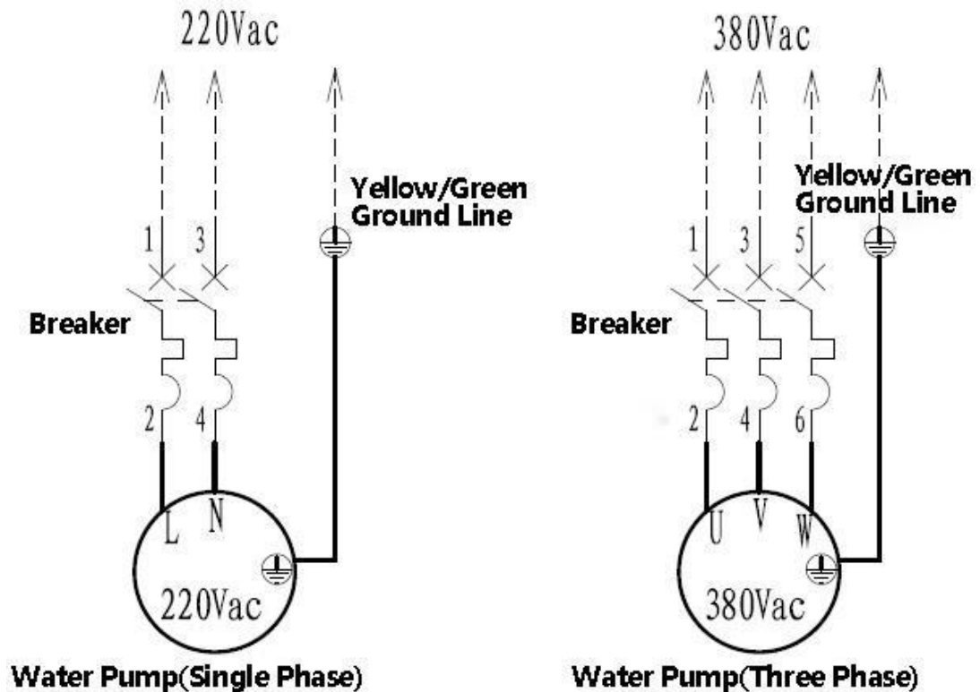
Water pump wiring diagram Fig 2-5
