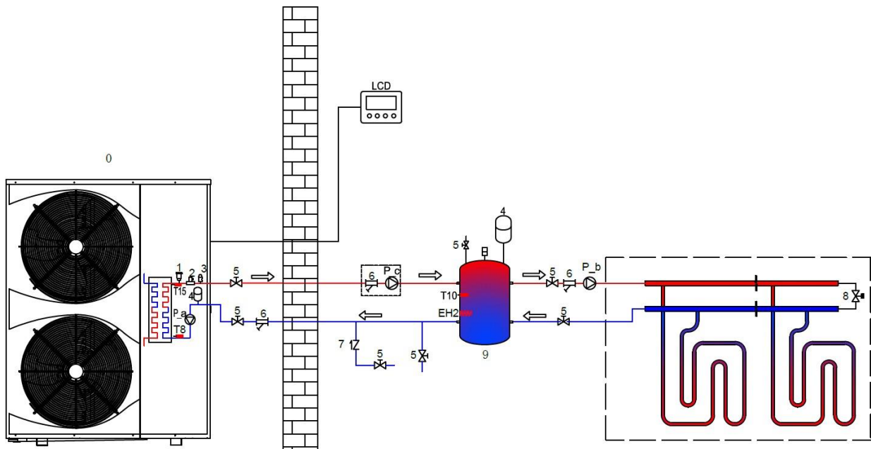
Installation diagram of the heating or cooling mode waterway system
