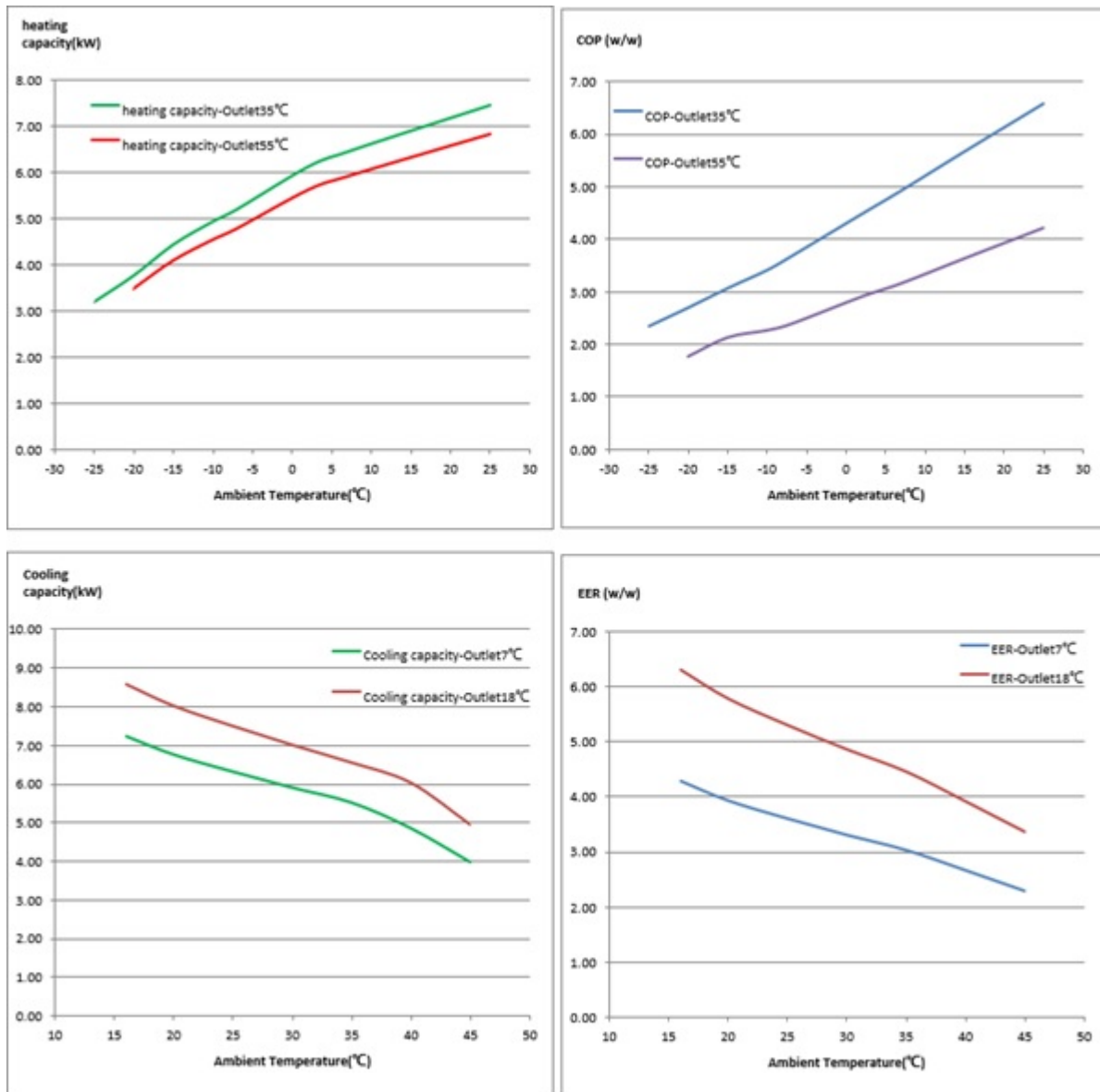
SOL-006HC1 Heating performance graph
