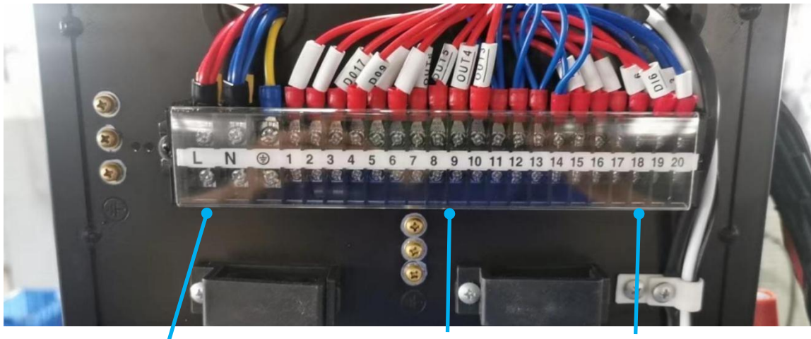
XT1 Power input 230VAC
